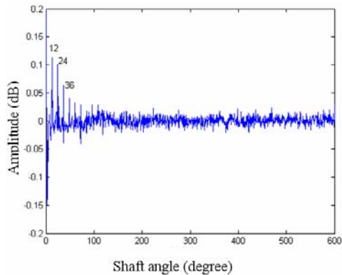
Fig. 9. Order cepstrum with normal condition.
