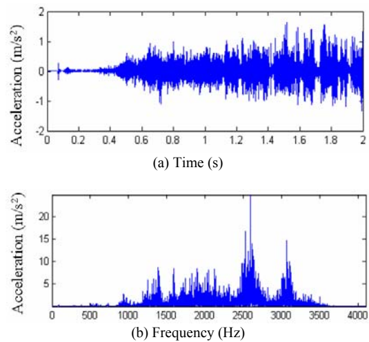
Fig. 4. Time-domain vibration signal with crack fault and FFT.
